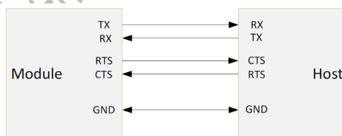
UART Connection
